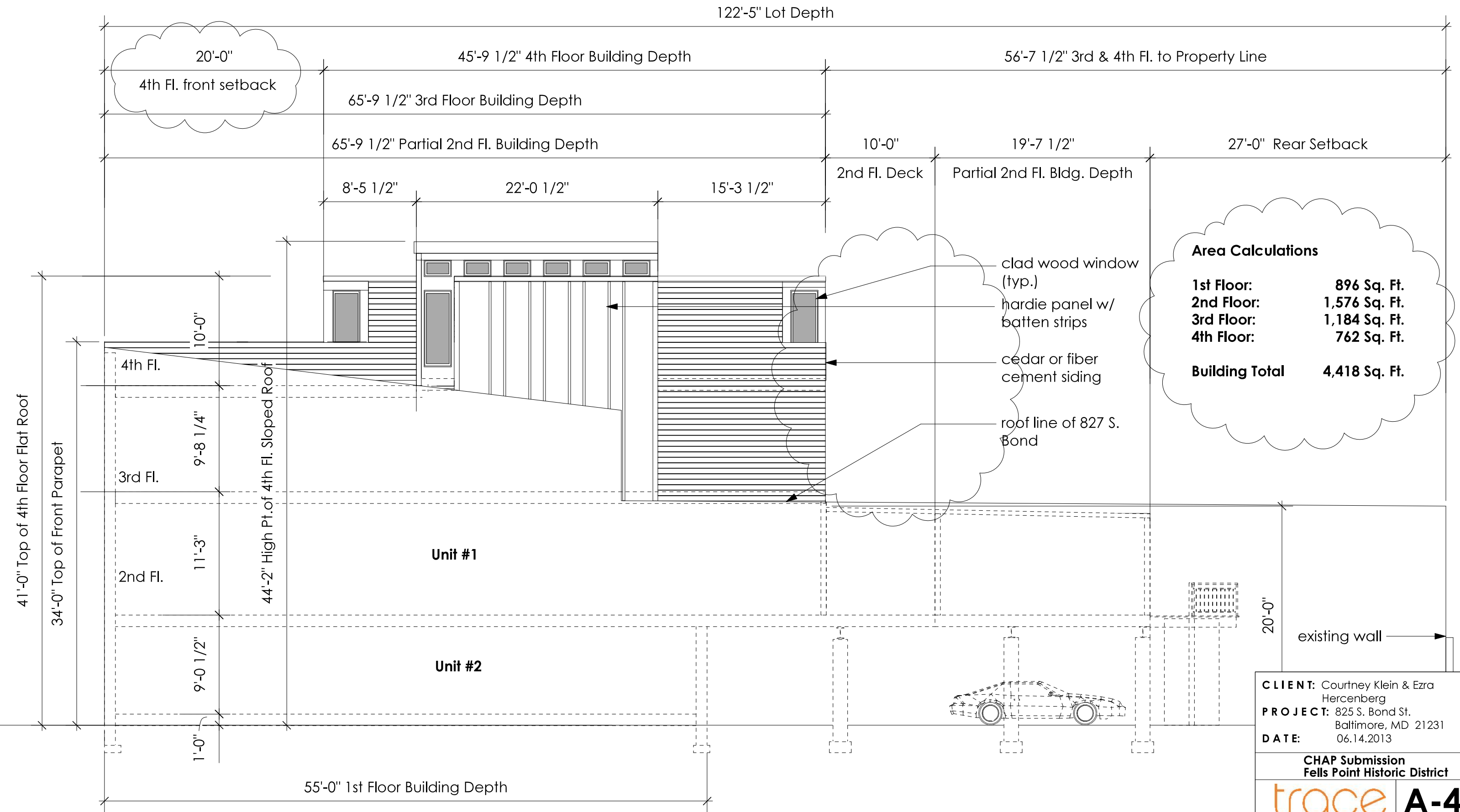
Revised Building Section Scale: 1/8" = 1'-0"
